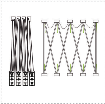
1. Stretch frame to size. Make sure webbing is not wrapped around grey locking arms.
